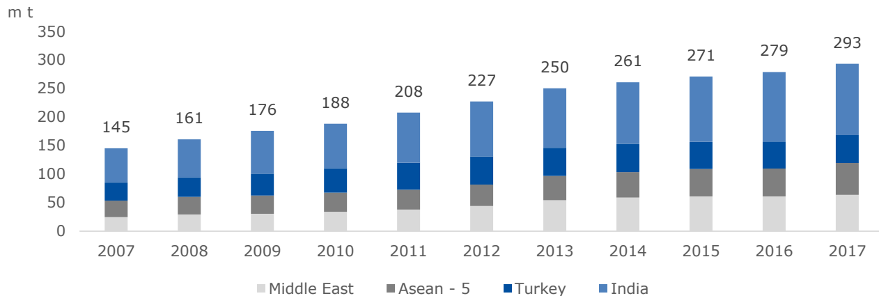
Steelmaking capacity evolution in developing countries - importers of steel
